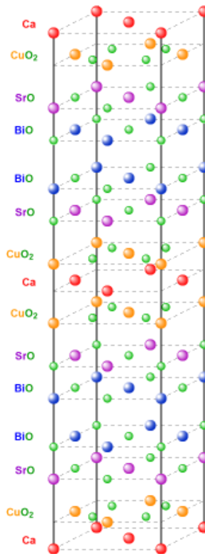
Figure 1. Structure of the crystallographic cell BSCCO-2212 [4].
