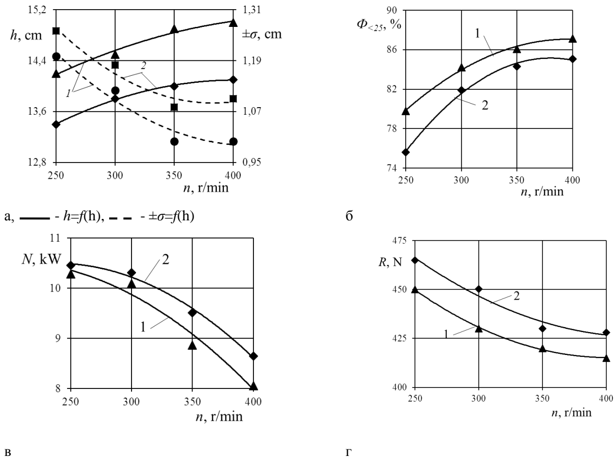
Fig.1. Influence of the number of revolutions of the rotary softener on the operating parameters of the device
