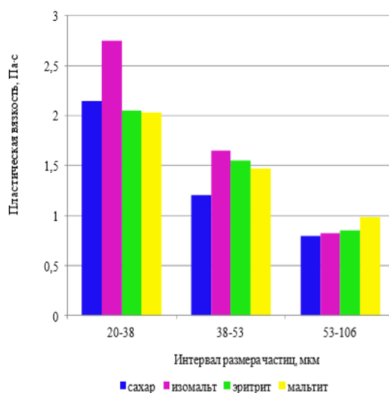
Figure 1. Plastic viscosity of chocolate samples in different particle size ranges
